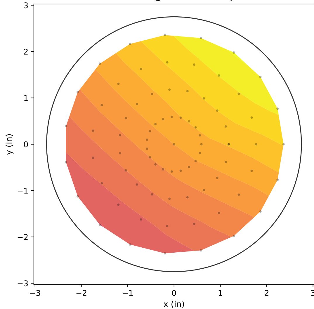
Slice 7 ( J=66.039 A/in 2 )
