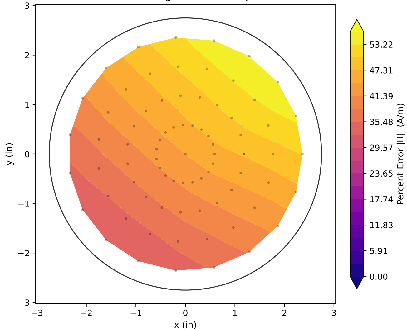
Slice 7 ( J=66.039 A/in 2 )
